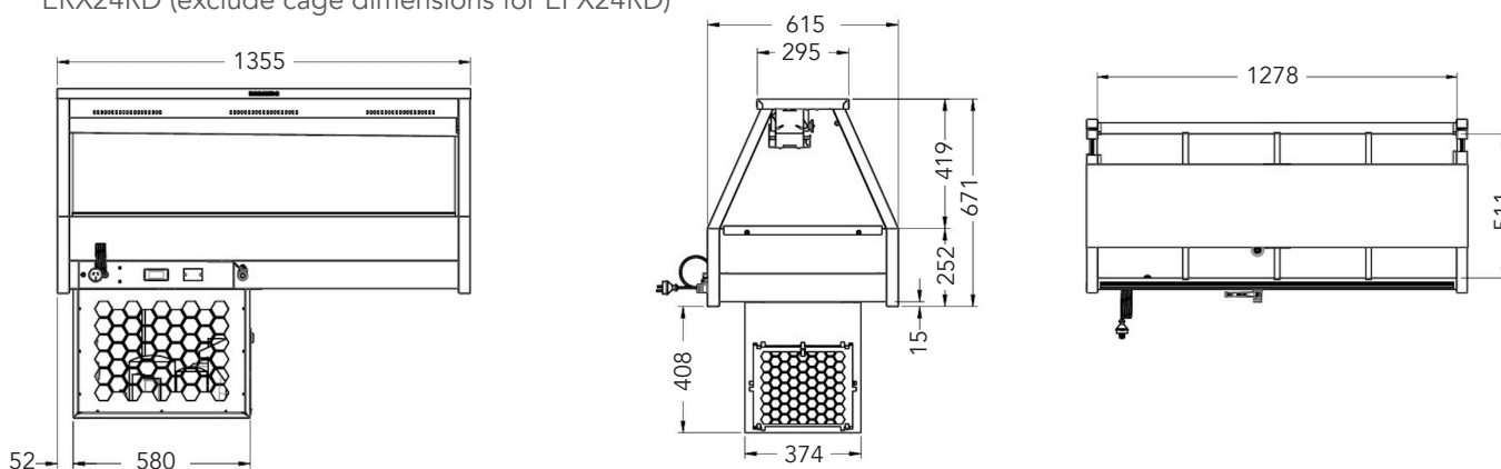
ERX25RD (exclude cage dimensions for EFX25RD)
